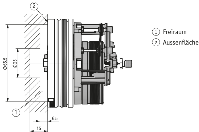
Abb. 3: Montagefreiraum
