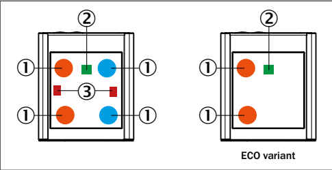
Fig. 8: Lighting unit ① Integrated lighting = 4 x LED (2 x left/2 x right); ECO variant: 2 x LED (2 x left) ② Feed-back spot (e.g. for Good Read) = 1 x green LED ③ Aiming laser for alignment, can be deactivated = 2 x red laser LEDs
