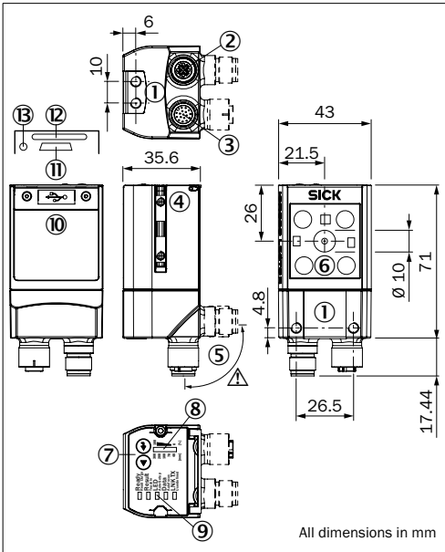
Fig. 6: Structure of Lector620 Professional, High Speed, DPM Plus and OCR ① M5 blind tapped holes, 5 mm deep (4 x), for mounting the Lector620 ② "Ethernet" connection (4-pin M12 female connector, D-coded) ③ "Power/Serial Data/CAN/I/O" connection (17-pin. M12 male connector, A-coded) ④ M5 sliding nuts, 5 mm deep (2 x), for mounting the Lector620 (alternative) ⑤ Swivel connector ⑥ Reading window ⑦ Function button (2 x) ⑧ Bar graph display ⑨ RGB LEDs for status indication (2 modes), 5 x ⑩ Cover (flap) ⑪ USB port, 5-pin female connector, Micro B type ⑫ Slot for microSD memory card ⑬ LED for microSD memory card
