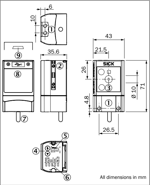
Fig. 7: Structure of Lector620 ECO ① M5 blind tapped holes, 5 mm deep (4 x), for mounting the Lector620 ② M5 sliding nuts, 5 mm deep (2 x), for mounting the Lector620 (alternative) ③ Reading window ④ Function button (2 x) ⑤ Bar graph display ⑥ RGB LEDs for status indication (2 modes), 5 x ⑦ Cable (0.9 m) with 15-pin D-Sub HD male connector ("Power/Serial Data/CAN/I/O") ⑧ Cover (flap) ⑨ USB port, 5-pin female connector, Micro B type
