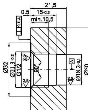
Fig.10d. Weldable fitting ring for use with transmitters with CG1/2 - type connector Material – 316Lss
