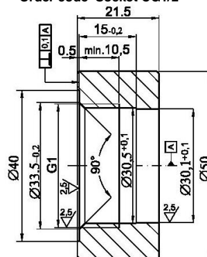
Fig.10f. Weldable fitting ring for use with transmitters with CG1 - type connector Material – 316Lss
