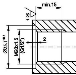
Fig.8b. Socket for P-type connector, (GP-type connector)
