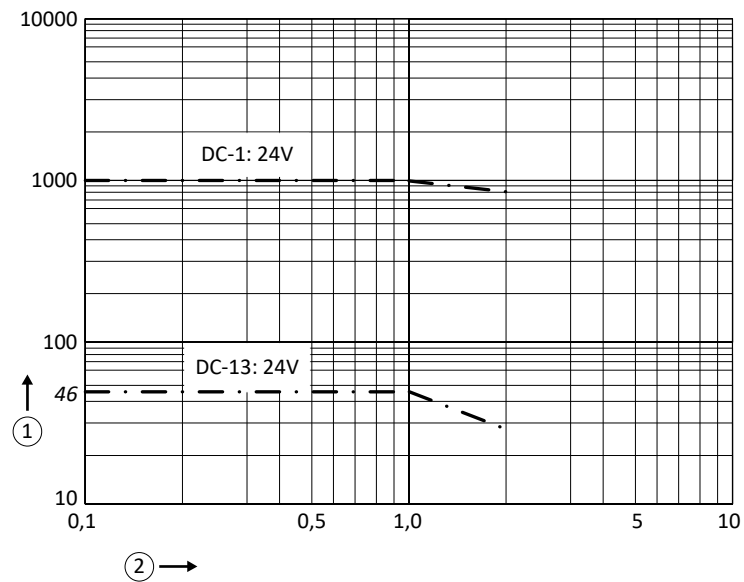
Figure 17: Electrical endurance of contacts 37/38
