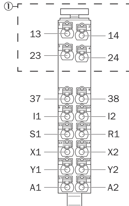
Figure 11: Terminals on front connector
