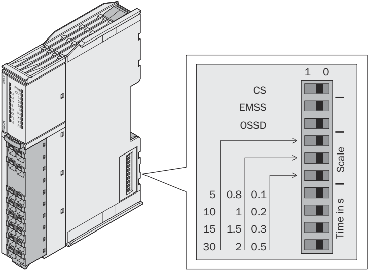
Figure 12: DIP switch
