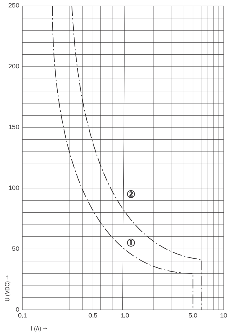
Figure 15: Breaking capacity without continuous arcing
