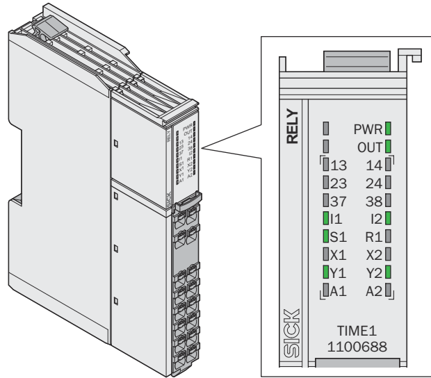
Figure 2: LEDs
