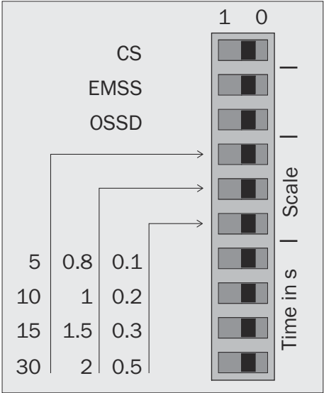
Figure 13: DIP switch release delay
