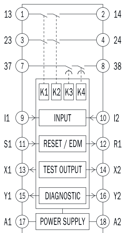
Figure 19: Internal circuitry
