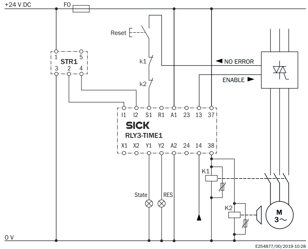
Figure 5: ReLy TIME1 connection diagram
