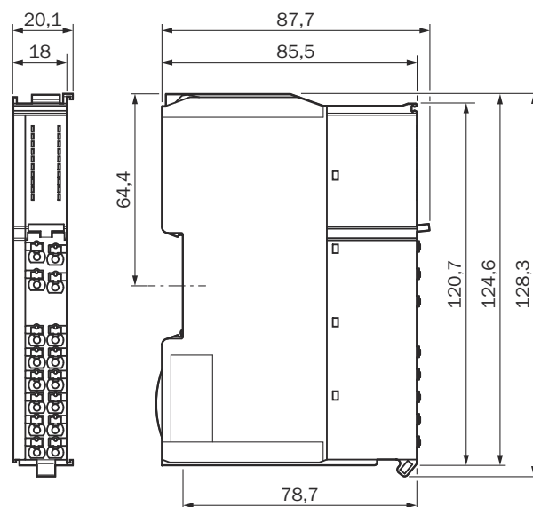
Figure 18: Dimensional drawing
