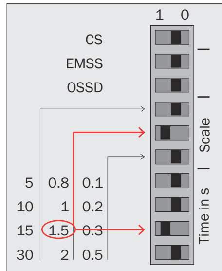
Figure 14: Release delay example
