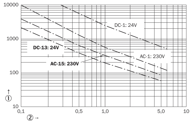
Figure 16: Electrical endurance of contacts 13/14 and 23/24
