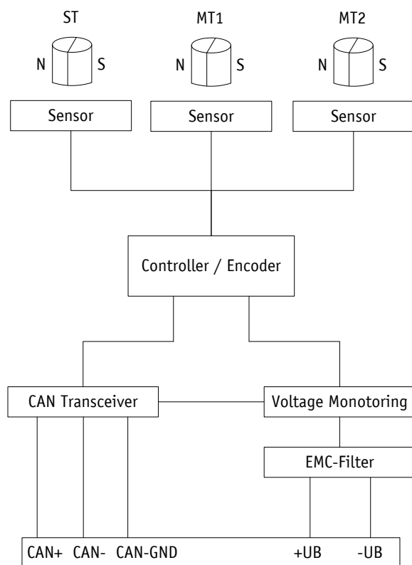
Fig. 2: Block diagram of non-redundant version
