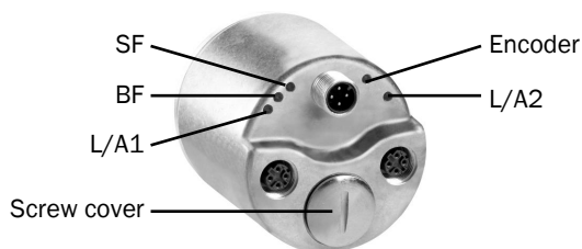
Figure 27: Position of the LEDs
