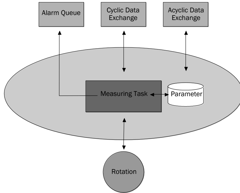
Figure 4: Encoder object model
