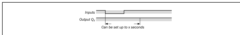
Fig. 29: Retriggering ON, with/without restart interlock
