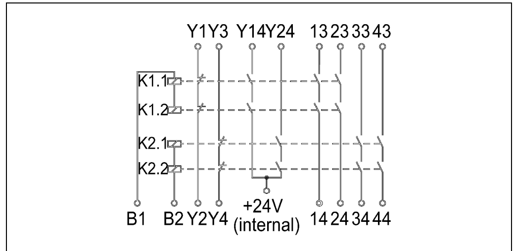
Fig. 14: Internal structure UE410-4R0
