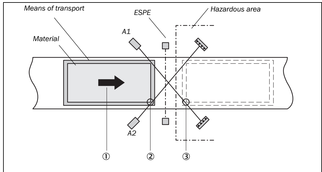
Fig. 23: Schematic layout
