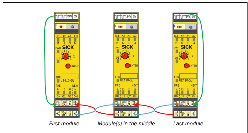
Fig. 9: Connecting several UE410-GU modules
