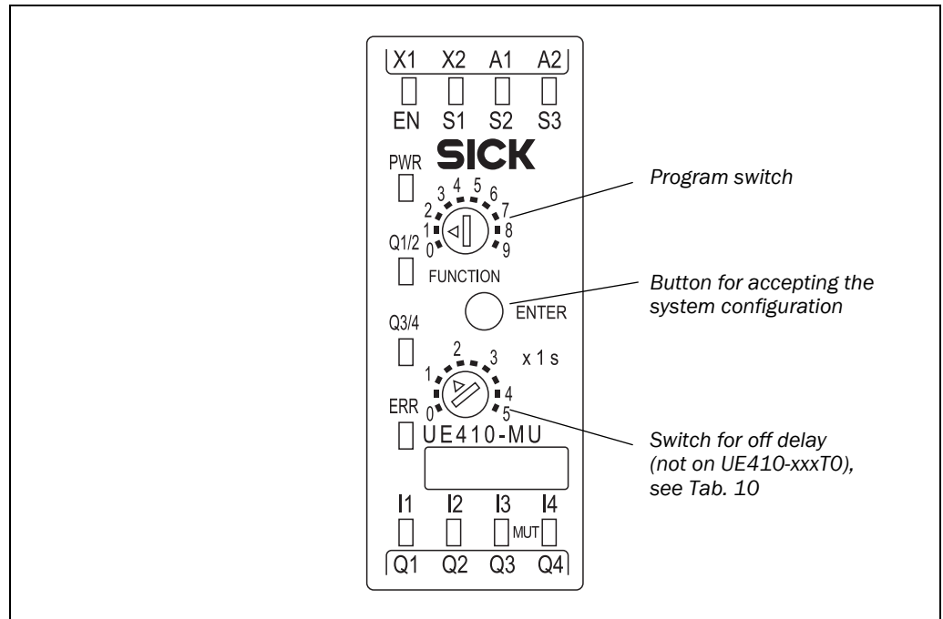
Fig. 7: UE410-MU controls and status indicators
