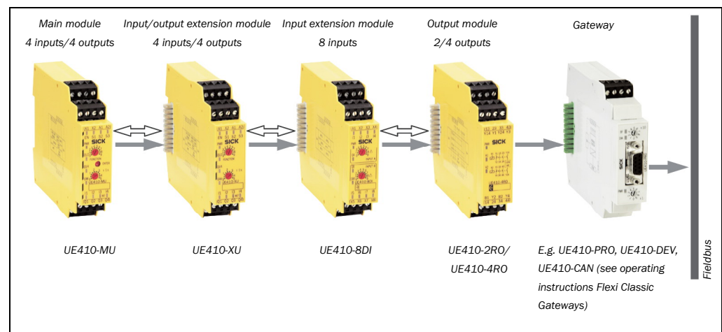
Fig. 2: Safety controller structure Flexi Classic (example with UE410-MU)
