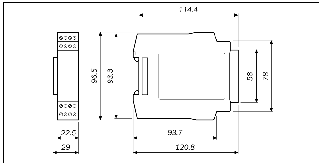
Fig. 51: Dimensional drawing UE410-XU, UE410-8DI, UE410-2RO, UE410-4RO, UE410-PRO, UE410-DEV, UE410-CAN (mm)
