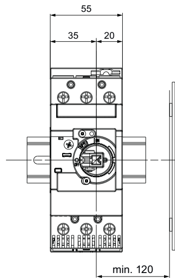
Figure C-32 3RV2.3
