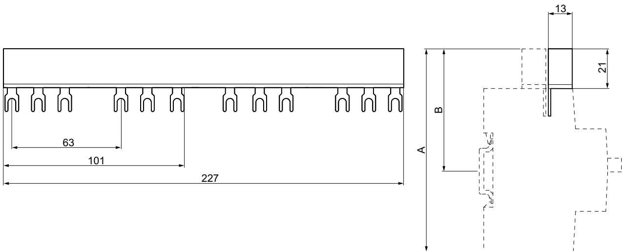
Figure C-21 3RV1915-3..
