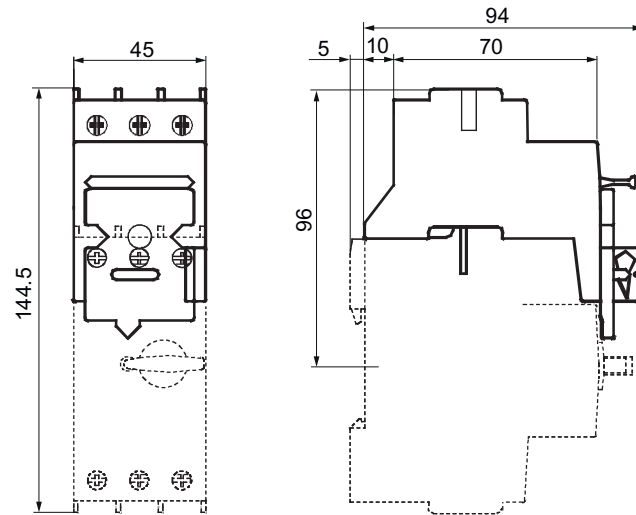
Figure C-17 3RV2928-1A
