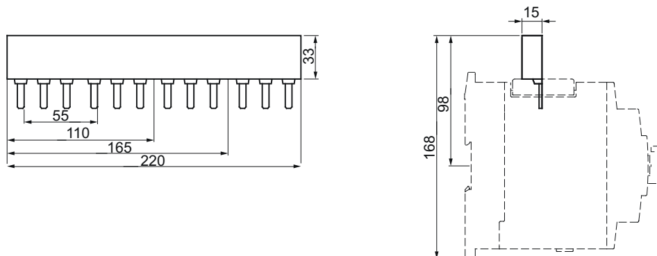
Figure C-22 3RV1935-1.
