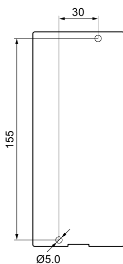
Figure C-16 3RV2.4 motor starter protectors
