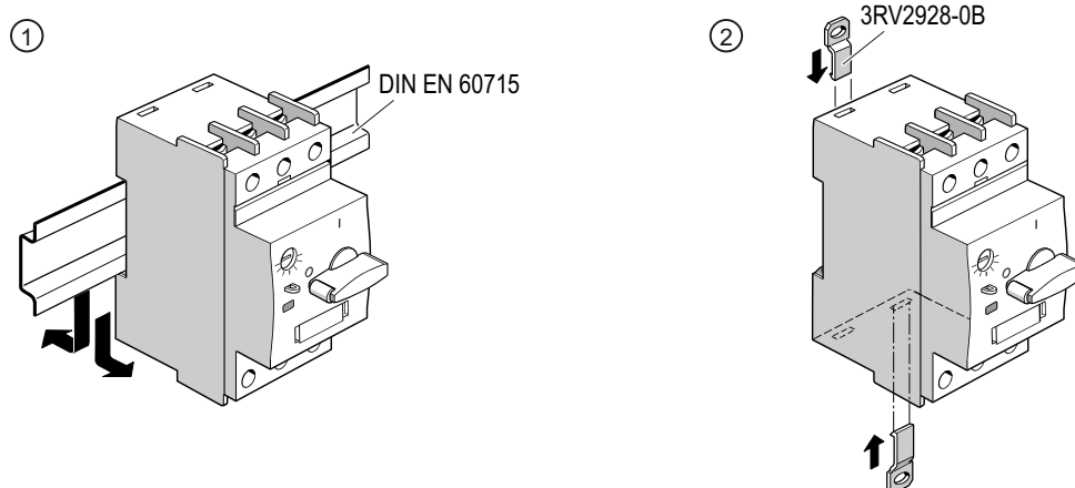
Figure 7-2 Mounting/disassembling motor starter protectors (sizes S00 and S0)
