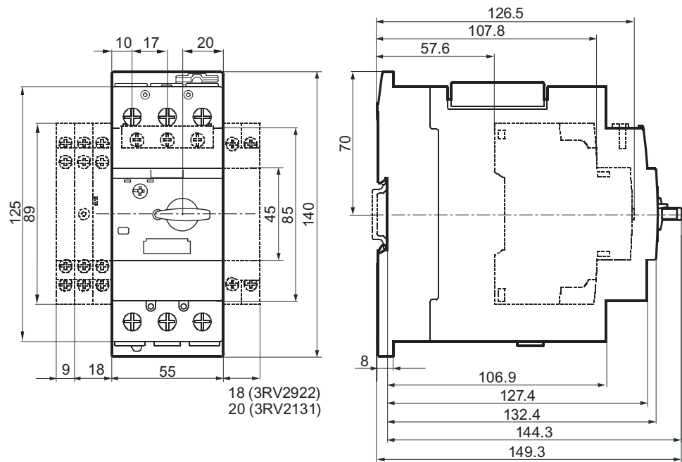
Figure C-11 3RV2.31 motor starter protector (≤ 45 A)
