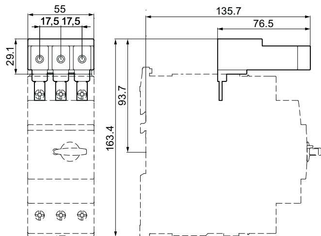
Figure C-27 3RV2935-5A
