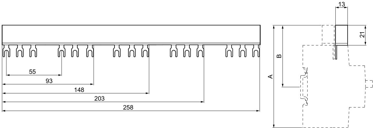
Figure C-20 3RV1915-2..
