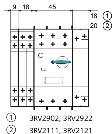
Figure C-4 Motor starter protectors with screw-type and spring-loaded connection, S00/S0
