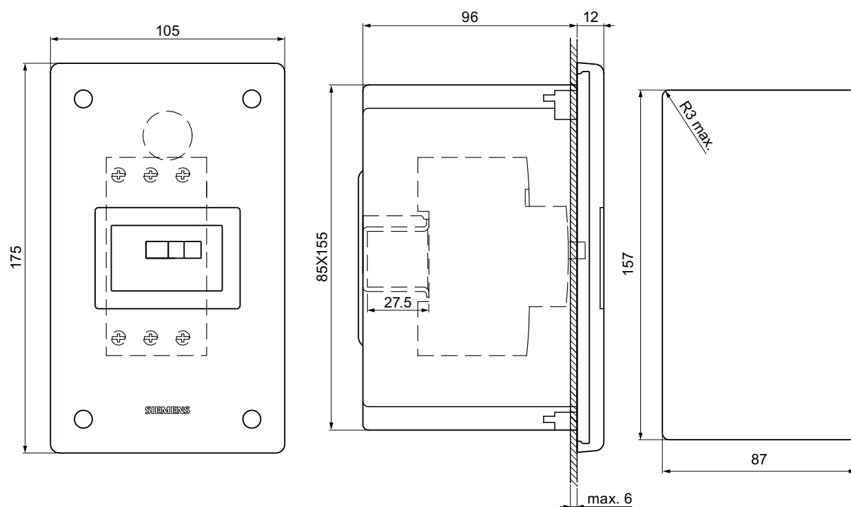
Figure C-42 3RV1913-2DA00
