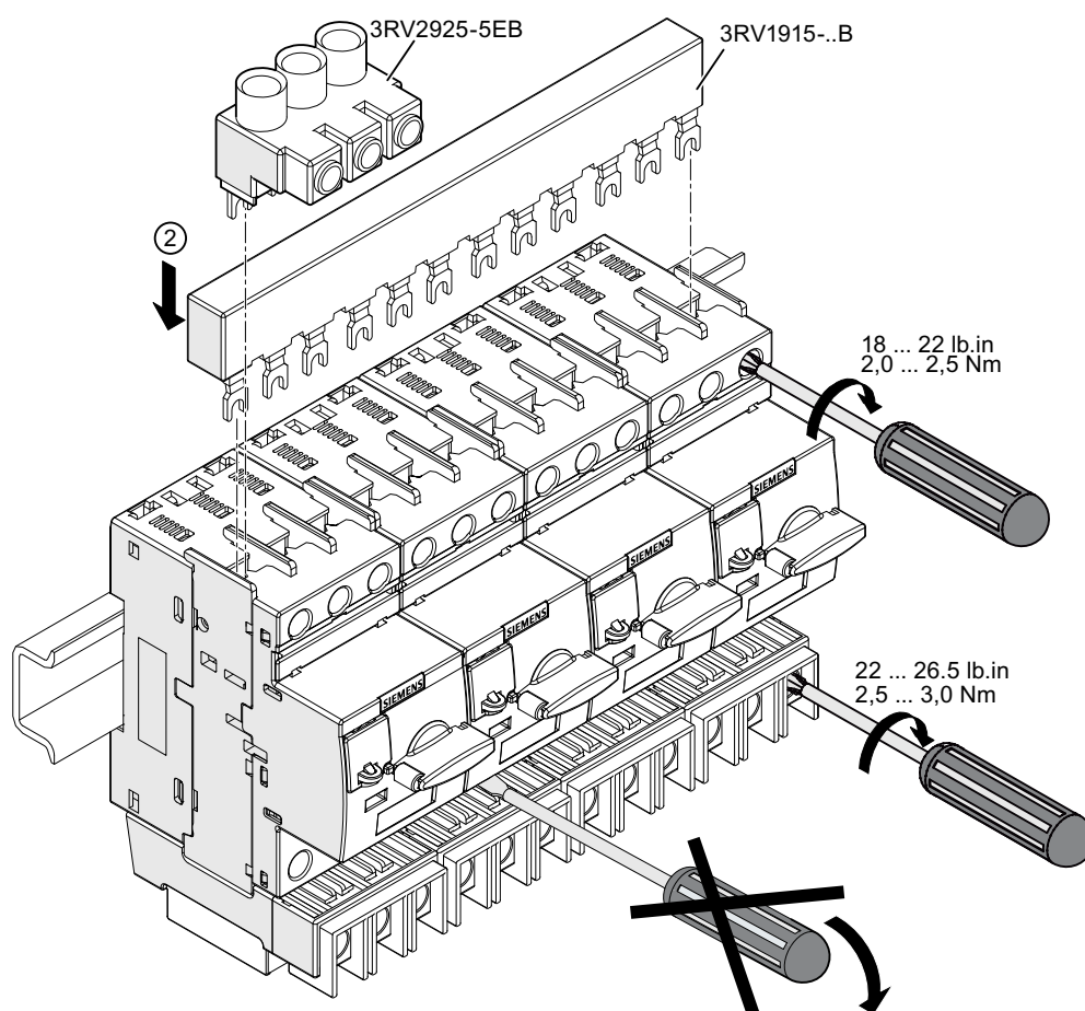
Figure 10-7 Installation with 3-phase busbars (3RV2711 / 3RV2721 / 3RV2811 / 3RV2821 size S00 / S0)
