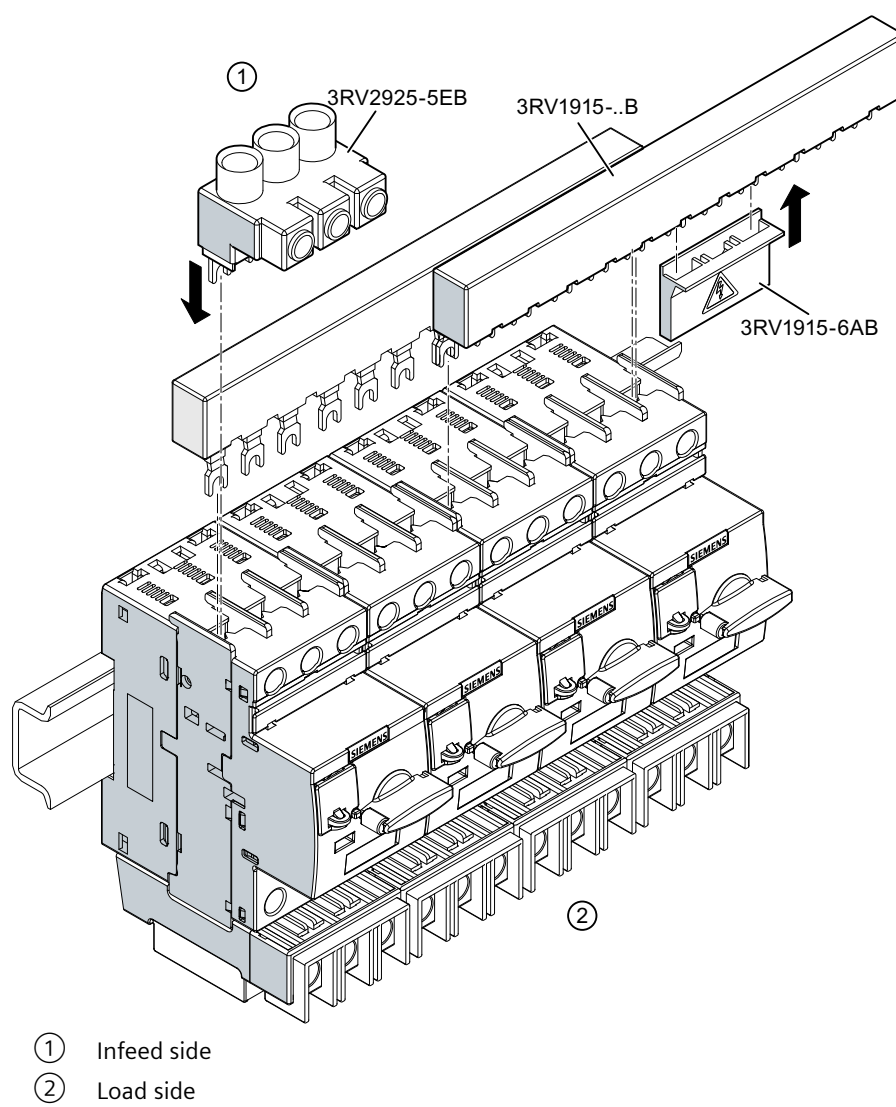
Figure 10-8 Installation with 3-phase busbars (3RV2711 / 3RV2721 / 3RV2811 / 3RV2821 size S00 / S0)
