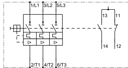
3RV1611-0BD10 3RV1611-1.G14
