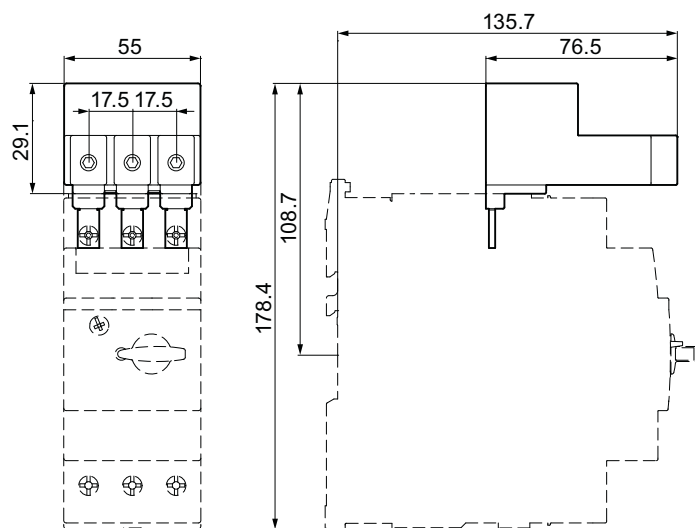
Figure C-28 3RV2935-5E
