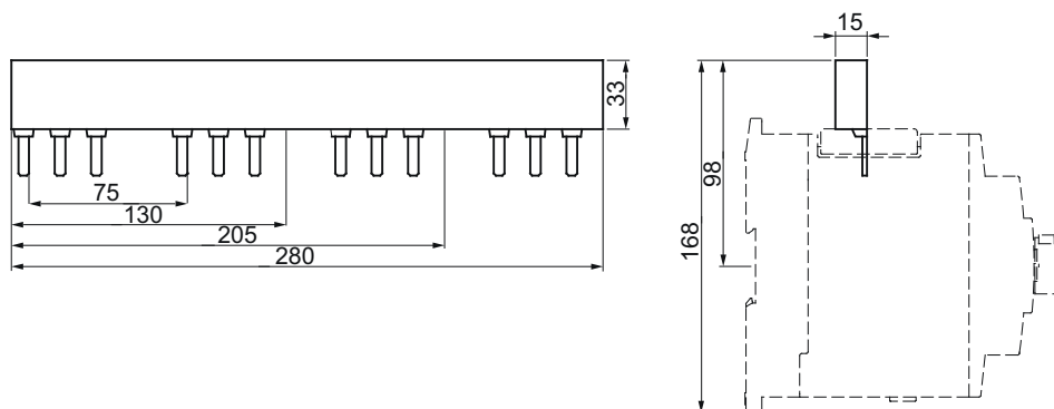
Figure C-23 3RV1935-3.
