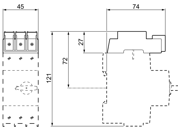
Figure C-34 3RV2928-1H
