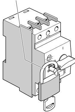
Figure 9-2 Securing the rotary switch (3RV2)
