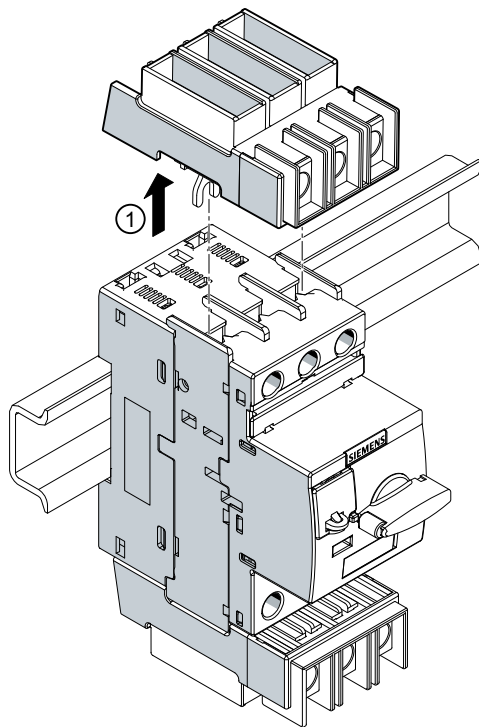
Figure 10-6 Installation with 3-phase busbars (3RV2711 / 3RV2721 / 3RV2811 / 3RV2821 size S00 / S0)
