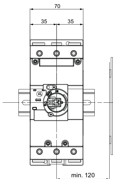
Figure C-33 3RV2.4
