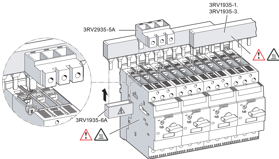
Figure 10-9 Mounting with 3-phase busbar (size S2)
