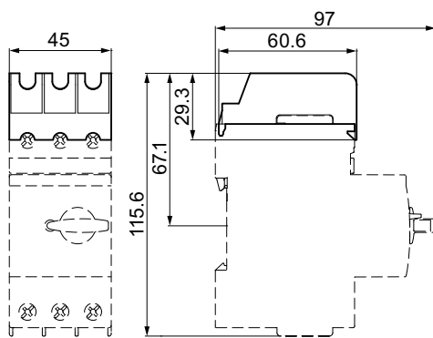
Figure C-35 3RV2928-1K
